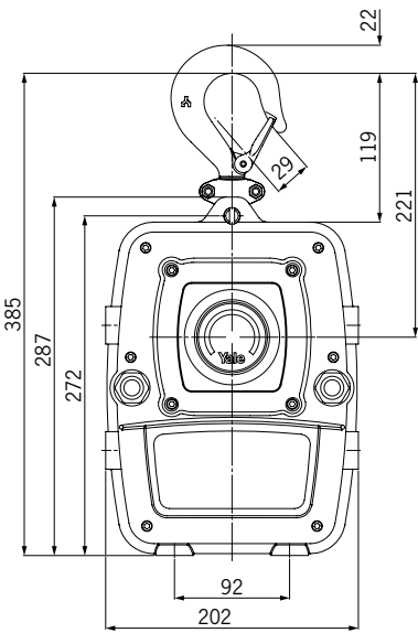
Yale Mtrac , 66 - 500 kg
